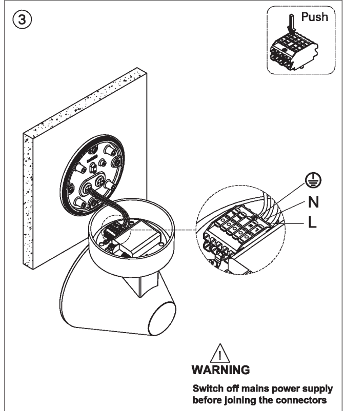
MOUNTING DETAIL
