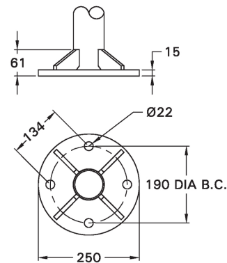
MOUNTING DETAIL
