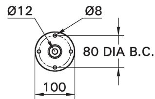
MOUNTING DETAIL
