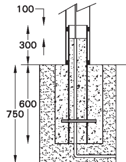
MOUNTING DETAIL
