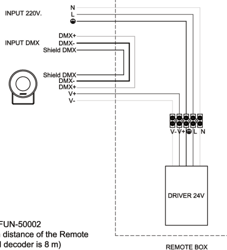
REMOTE BOX
