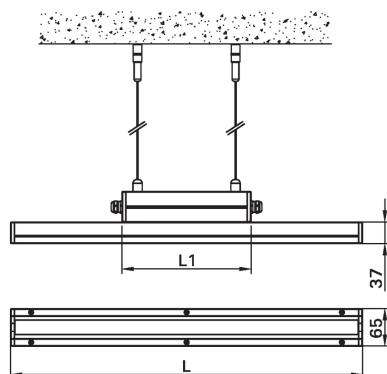
Mounting detail
