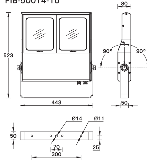
MOUNTING DETAIL
