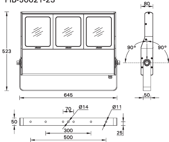
MOUNTING DETAIL
