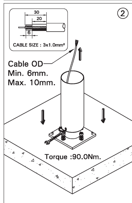
MOUNTING DETAIL
