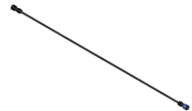
Cable - Connector IP67 Female + Male 3 Pin Power - Length 5000 mm A67891-005
